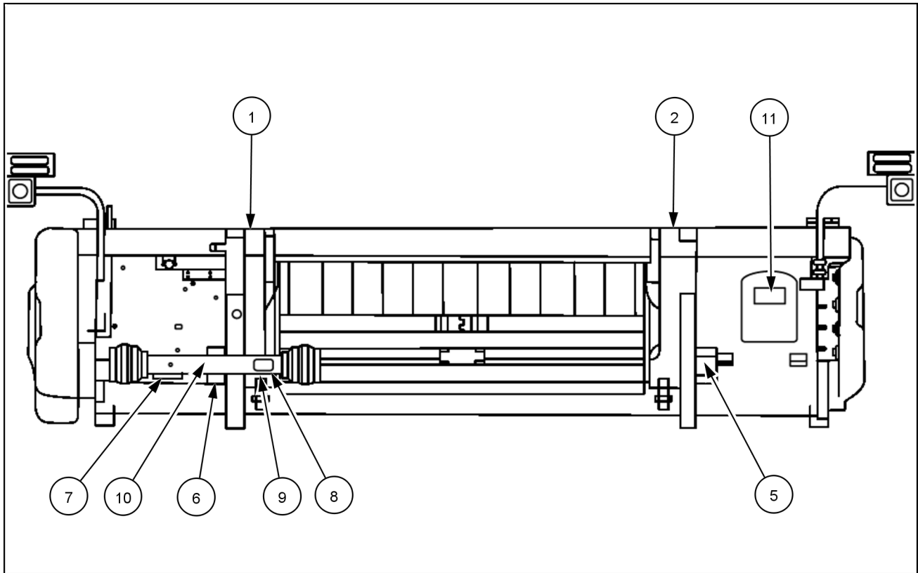
Rear view
